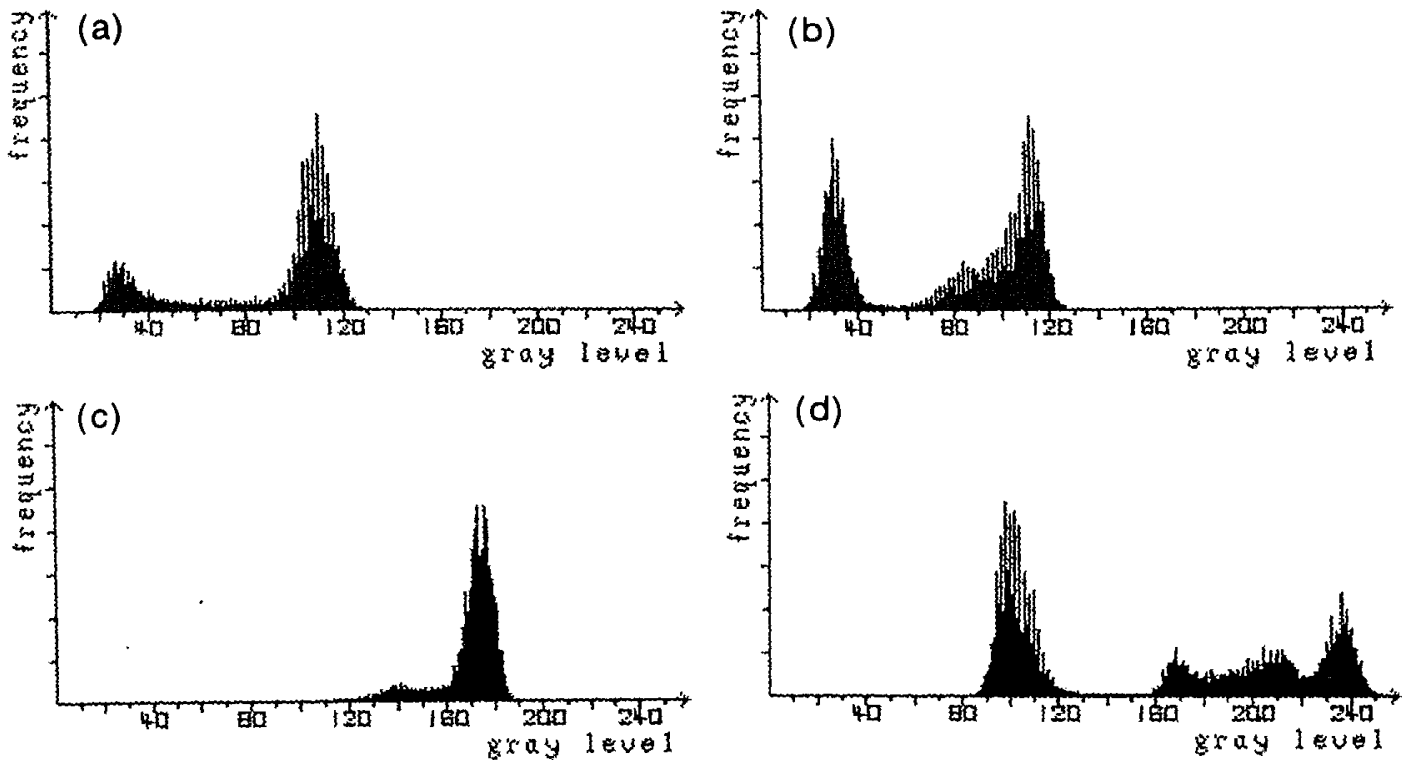
Fig. 2. The gray-level histograms for images of Fig. 1: (a) "dragon" image; (b) "gear" image; (c) "dragon text" image; (d) "coin" image.
