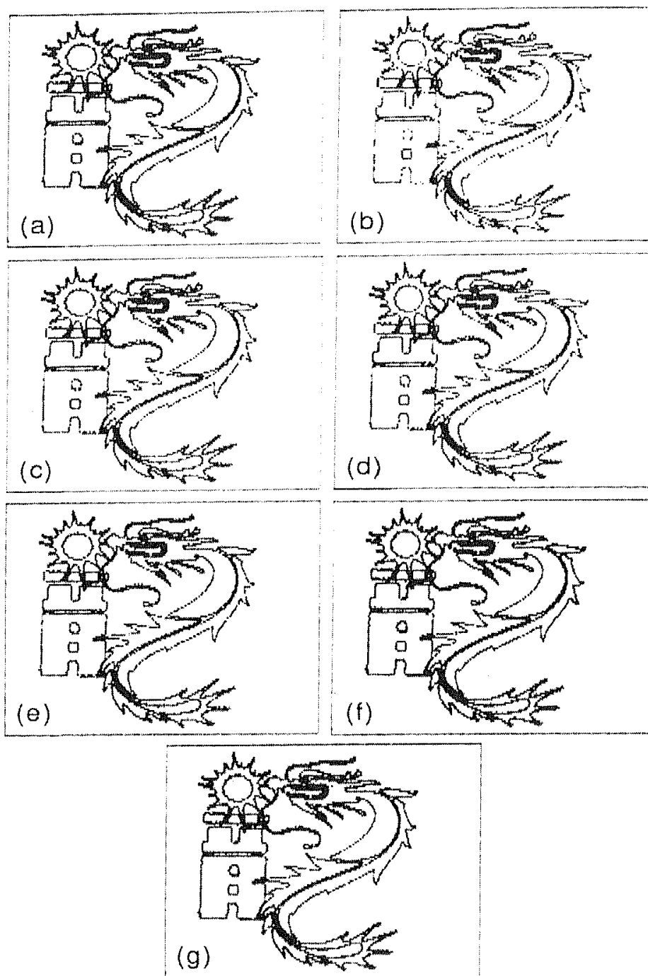
Fig. 5. The binary images of Fig. 1(c) tested by the methods considered: (a) E ; (b) E^* ; (c) \eta ; (d) \eta^* ; (e) Otsu method; (f) moment-preserving method; (g) minimum error method.
